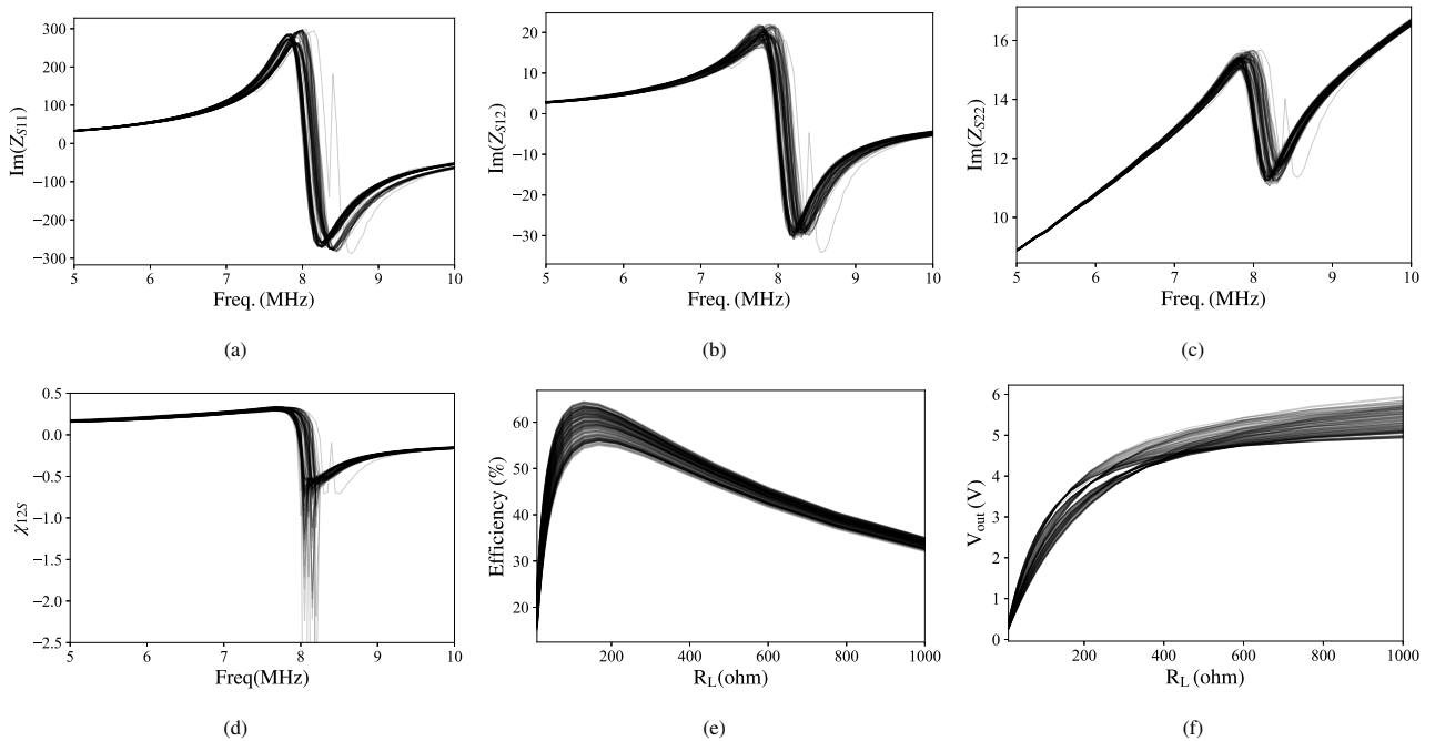
Figure 10. (a), (b), (c), elements of the measured impedance matrix of the coupled inductors, indexes 1 and 2 correspond to the Tx and Rx port, respectively, (d) generalized coupling coefficient (11), (e) efficiency (12) and (f) output voltage (with V_{in} = 1V ). Each line, partly transparent to express a density, corresponds to a different Rx position: 130 positions with 1 mm step are considered, from the Rx aligned with the first Tx, to the Rx aligned with the fifth Tx. In (a)–(d) the compensating capacitors have been shorted.
