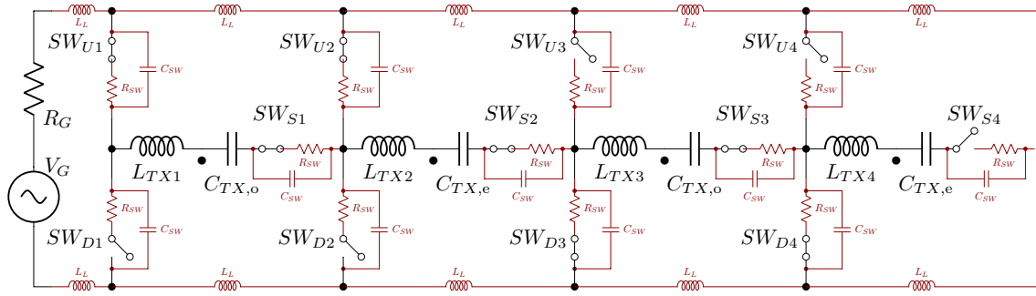
Figure 11. Simulated layout of State A (equivalent to Fig. 4) with line stray inductances ( L_L = 20 nH), switch stray capacitances ( C_{SW} = 200 pF) and loss resistances ( R_{SW} = 100 m \Omega ). The Rx is not shown but included in the simulation as ideal. The other intermediate states are obtained by the proper selection of the switches.
