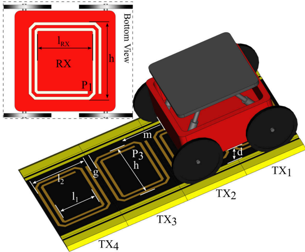
Figure 1. Sketch of a wireless powered mover, with a sequence of transmitters and one receiver; only two transmitters are active at a time. P_1, P_2 (on TX 2 , covered by the RX), P_3 are the WPT-link ports; d is the Tx-to-Rx distance; h, l_1 and l_2 are the Tx-coil geometrical parameters; g is the distance between the Tx-coils; l_{RX} is the Rx coil length; m is the Rx-to-Tx displacement. Dimensions of the designed and measured prototype (mm): l_1 = 20, l_2 = 30, h = 40, d = 10, l_{RX} = 28.5, g = 3.5 .
