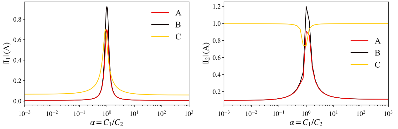
Figure 8. Magnitude of I_1 and I_2 when the system is in states A, B, and C. In state A the magnitude of I_3 is equal to the magnitude of I_1 .
