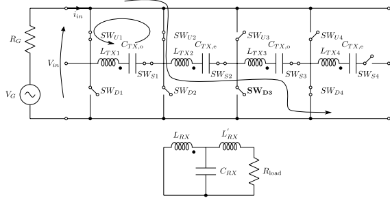
Figure 7. Temporary states due to the not synchronous commutation of the switches, the switch SW_{D3} gets open before SW_{U1} and SW_{S1} (“State C”).
