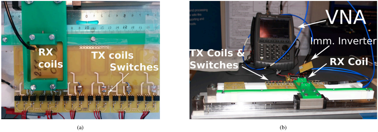
Figure 9. System to be measured: (a), a top view of the system and (b), the complete set-up to be measured.
