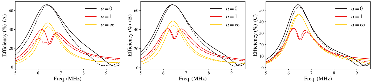
Figure 12. Measured (solid lines) and simulated (Ac analysis, dashed lines) efficiency with the system in state A, B and C.
