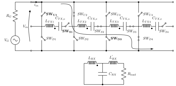
Figure 4. Circuit representation of the modular WPT link when the Rx coil is located between the second and the third Tx coils: the associated current path is outlined.
