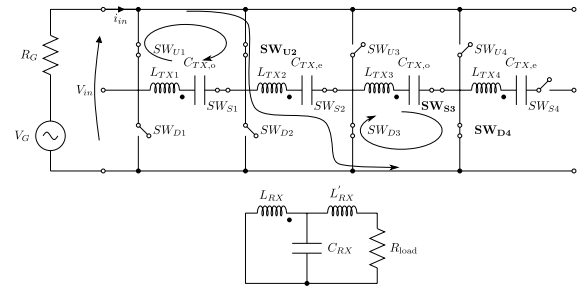
Figure 5. Intermediate state required to maintain current continuity (“State A”). The switches SW_{U2} , SW_{S3} , SW_{D4} are closed, before SW_{U1} , SW_{S1} , SW_{D3} are opened. Two potentially critical closed loops are created.
