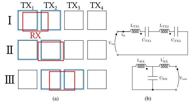
Figure 2. (a) outline of the movement, (b) equivalent 2-port of the moving link with two Tx coils in series.
