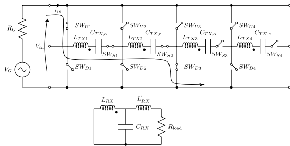
Figure 3. Equivalent circuit of the modular WPT link: two subsequent couples of the Tx coil are shown with the Rx located between the first two Tx coils, see Fig. 2(a) (I). The current path is outlined.
